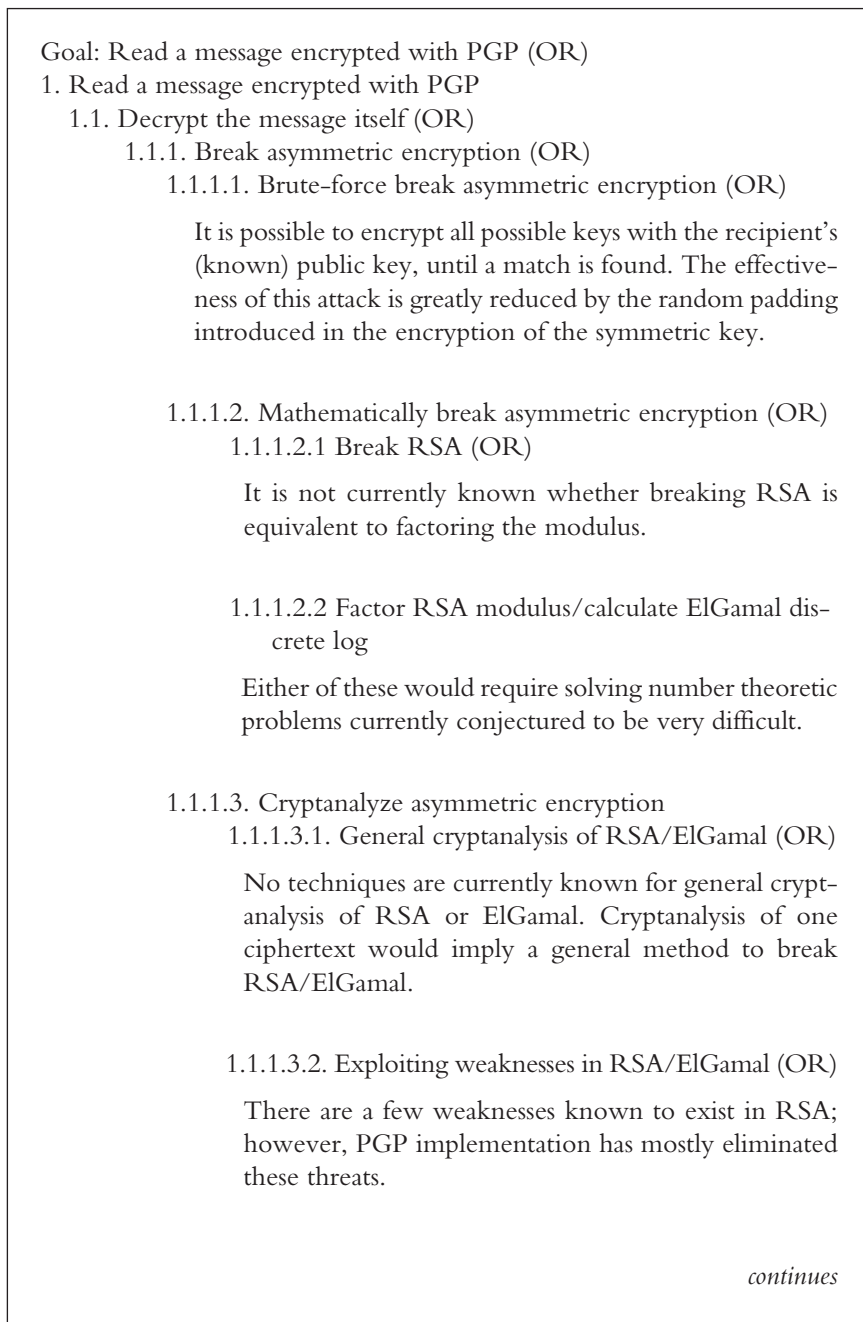
Figure 21.7 PGP attack tree
