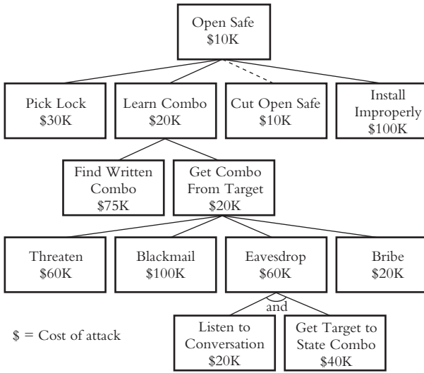
Figure 21.4 Cost of attack.
