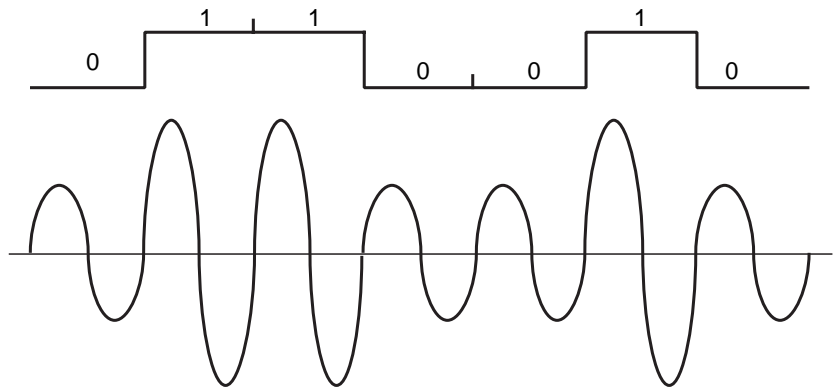
Figure 6.5 Modulation d'amplitude
