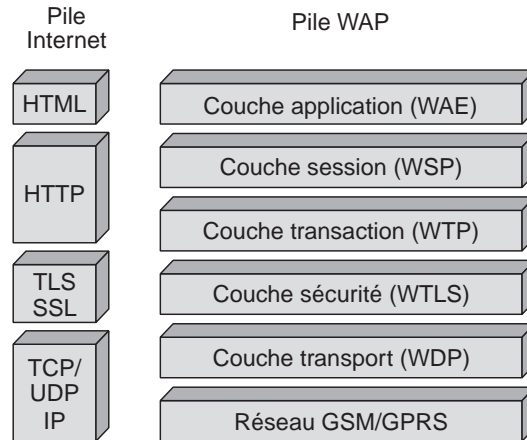
Figure 43.10 Architecture protocolaire du WAP
