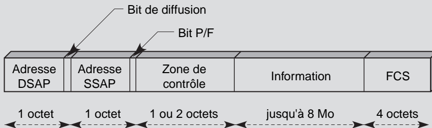
Figure 7.16 Format de la trame LLC
