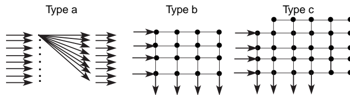
Figure 31.5 Commutateurs Crossbar
