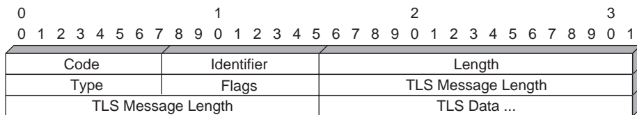
Figure 39.24 Paquet EAP/TLS
