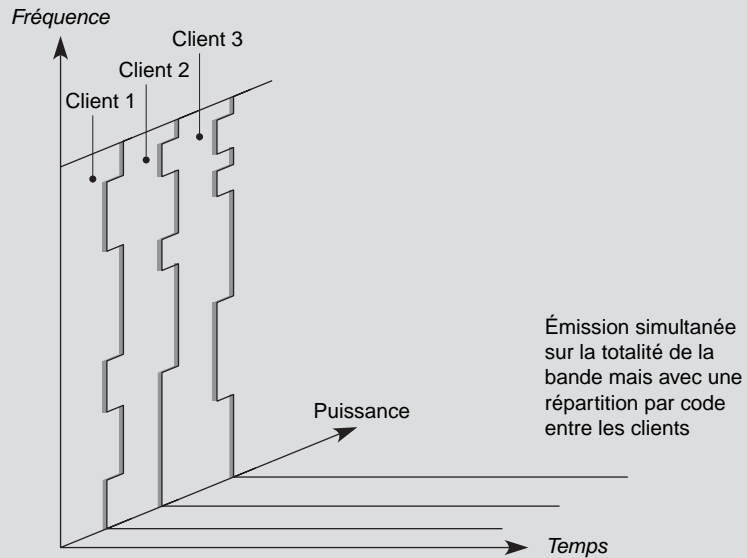
Figure 12.5 Le CDMA
