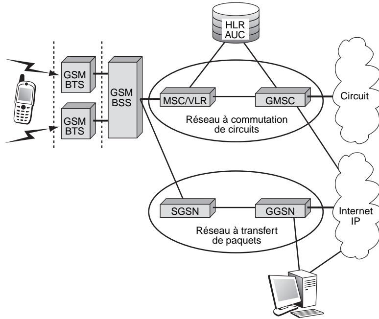
Figure 43.2 Architecture du GPRS
