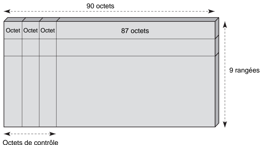
Figure 14.4 Trame SONET de base
