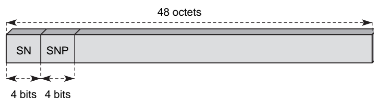
Figure 15.22 SAR-PDU de type 1
