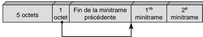
Figure 41.3 Cellule AAL-2
