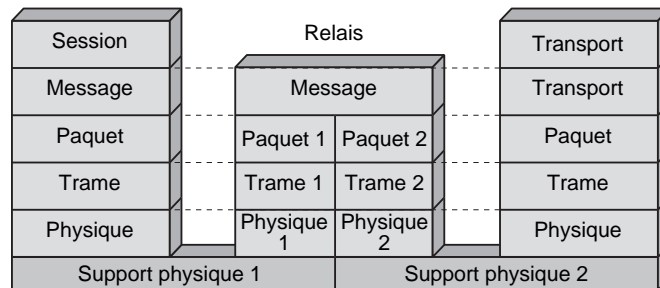
Figure 32.4 Architecture d'un relais
