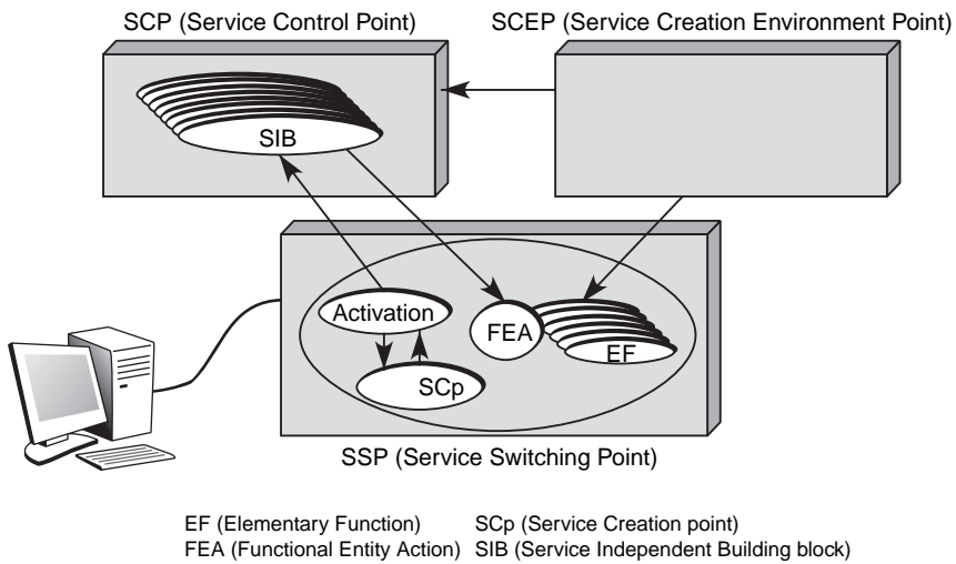
Figure 44.15 Architecture IN/2
