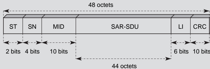
Figure 15.26 SAR-PDU de type 3/4
