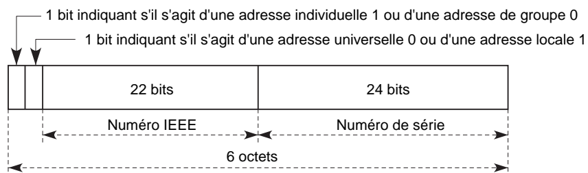
Figure 8.12 Adressage Ethernet
