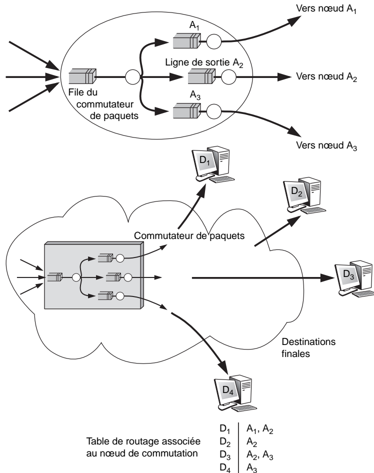
Figure 8.9 Table de routage
