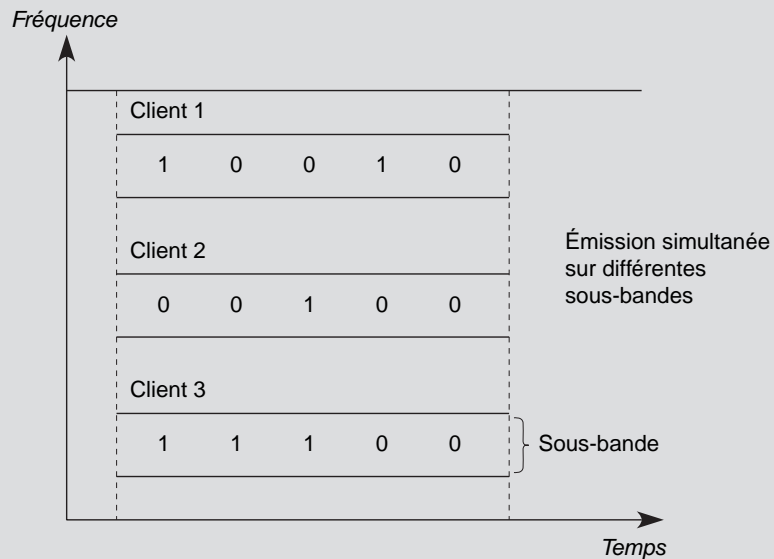
Figure 12.3 Le FDMA
