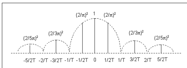
Figure 8.25: PiFM Harmonic Emissions
