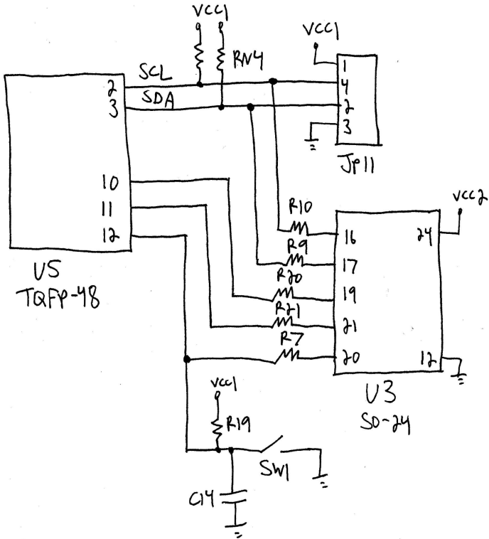
Figure 6.23: Schematic derived from Figure 6.22.
