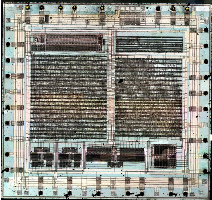
Figure 4.11: This is the complete die photograph of the Clipper Chip at reduced resolution.
