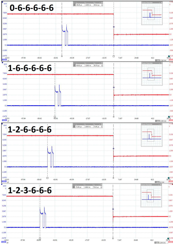
Figure 4.13: Disk Pin Timing Results
