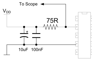
Figure 4.15: Tapping VCC for Power Analysis
