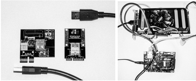
Figure 5.3: PCIe Adapters
