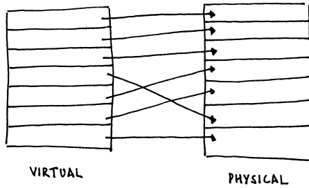
Figure 4.1: Virtual Memory
