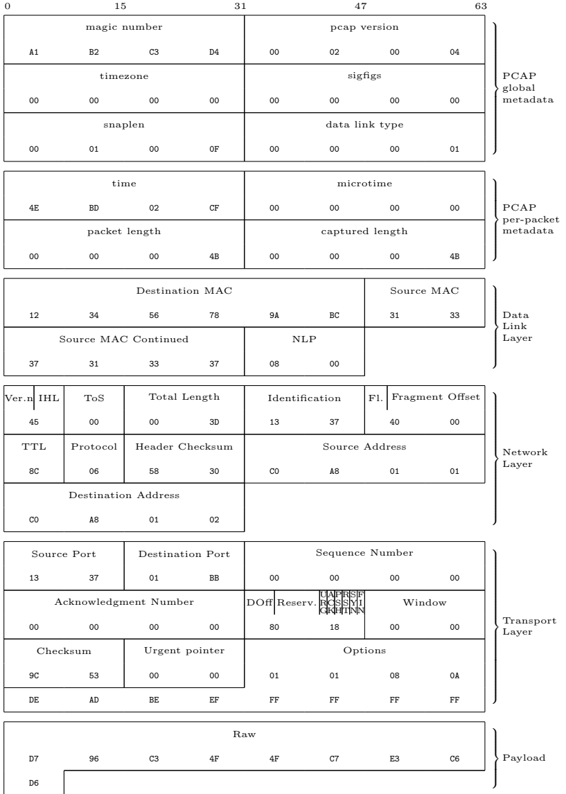
Figure 7.3: Crafted PCAP
