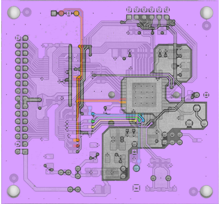
Figure 6.22: Layer stack-up of our example PCB. Layer opacity was adjusted to see through the board and arbitrary traces were colored using a flood fill.
