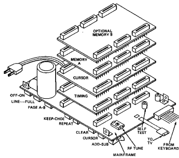
Figure 1.2: Don Lancaster's 1973 TV Typewriter
