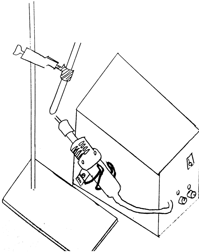
Figure 4.8: The clamp stand holds the test-tube next to the SMD rework station.
