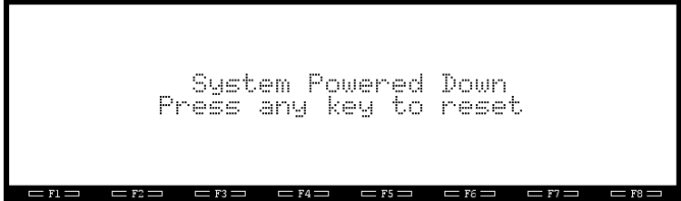
Figure 2.3: POKE 62975, 0
