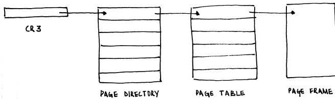
Figure 4.2: X86 Paging
