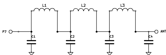
Figure 8.23: Lowpass Filter for Reducing PiFM Harmonics
