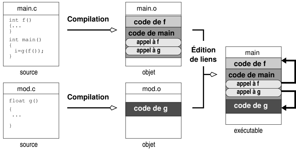
FIGURE 5.2 – Compilation séparée
