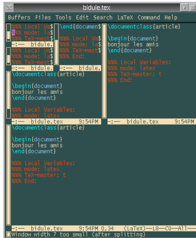
FIGURE 6.2 – The Emacs quad tree
